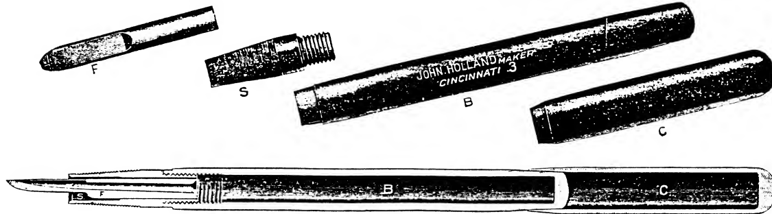
Bisected view of the John Holland Fountain Pen, the parts being in their proper position. F—Feed. S—Section. B—Barrel. C—Cap.
